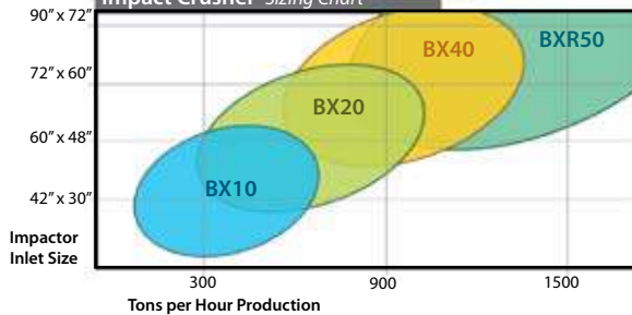
Impact Crusher Sizing Chart
