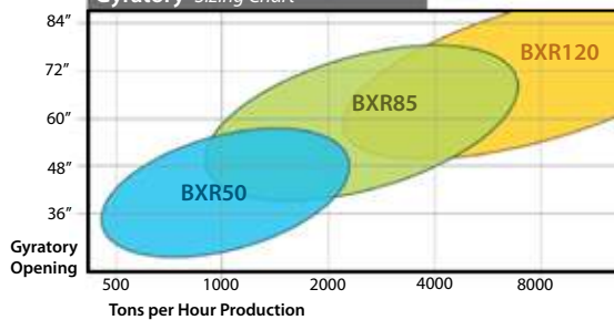
Gyratory Sizing Chart
